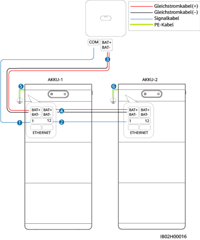
Abbildung 5-1 ESS-Kabelanschlüsse
