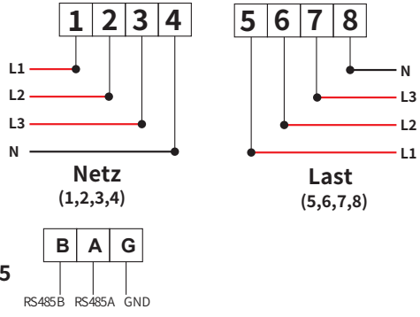
Abb. 7.20 EASTRON-Messer
